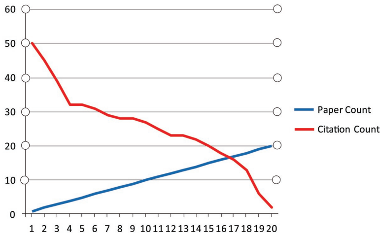
FIGURE 5.1: Illustrating h-index: an author’s h-index is when the publication count line crosses the citation curve, given that the papers are sorted from more to less on the X-axis.
