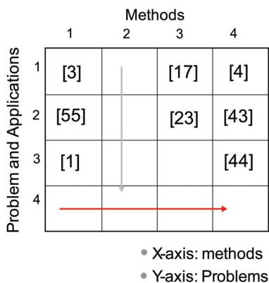
FIGURE 4.1: The research matrix method.
